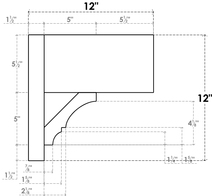
SIDE PROFILE
